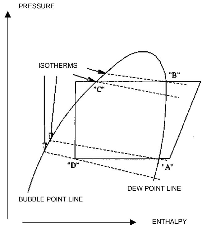
Pressure-Enthalpy Diagram for Non-azeotropic Refrigerant Blends
